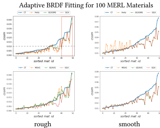
Figure 4: CSSIM error for each model fitted with the adaptive image-based BRDF fits.
