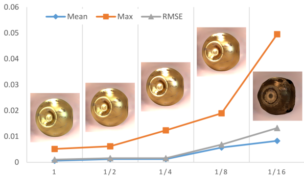
Figure 13: Impact of Rotation Speed. Relative Hausdorff distance (normalized by the length of the largest bounding box axis) for mean, maximum and RMS error on the recovered geometry for a temporally subsampled sequence mimicking different object rotation speeds with a fixed camera exposure.
