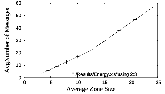
Fig. 5. Variation of message overhead with zone size
