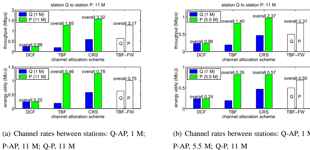
Fig. 7. The throughput and energy utility of stations under different channel allocation schemes (1 proxy and 3 clients)
