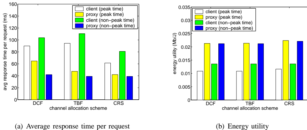
Fig. 10. Average response time per request and energy utility in BU Web client traces
