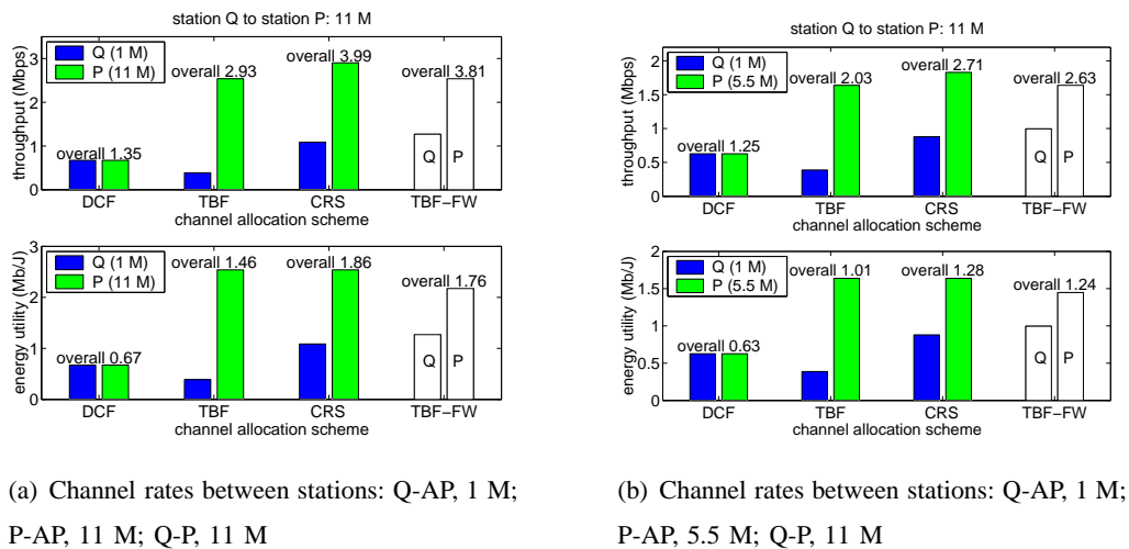
Fig. 6. The throughput and energy utility of stations under different channel allocation schemes (1 proxy and 1 client)
