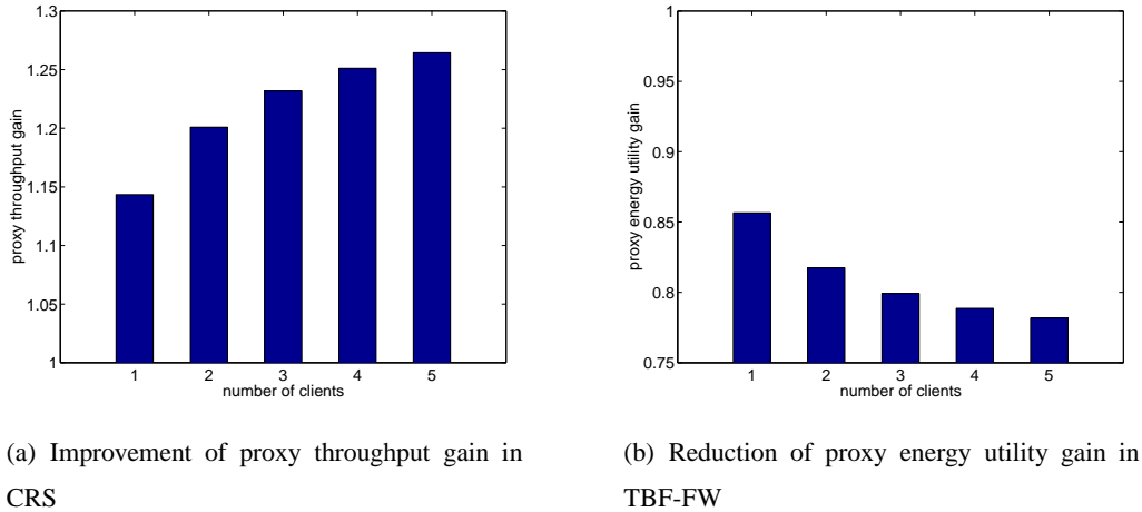
Fig. 9. Performance gain of proxy with different number of clients
