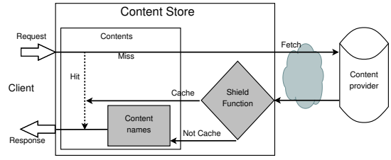
Fig. 1. CacheShield Structure.
