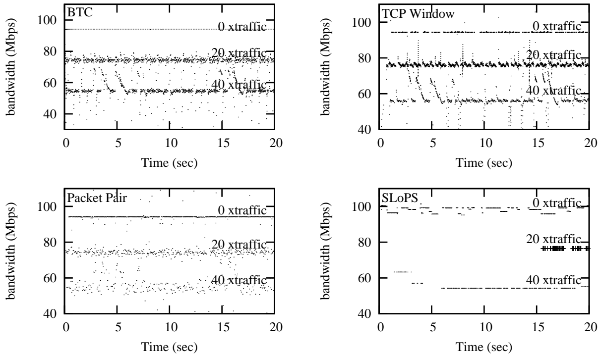
Figure 4. Techniques applied to iperf traces on a 100Mb LAN with 0,20,40 Mb of cross traffic.
