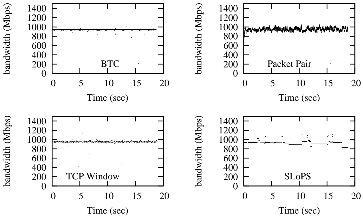
Figure 2. Techniques applied to iperf traffic monitored on uncongested 1 Gb LAN.
