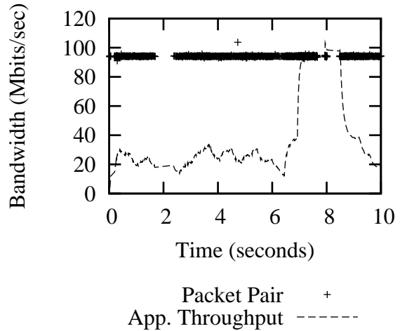
Figure 5. Throughput of an adaptive eigensolver measured on a 100 Mb LAN. This application has a bursty traffic pattern with a maximum rate obtained only between 6-9 seconds, but the packet pair technique is able to provide effective measurements throughout the duration of the trace.
