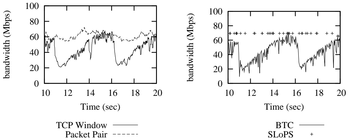
Figure 3. Techniques applied to trace of iperf traffic on a 100Mb WAN between W&M and CMU.
