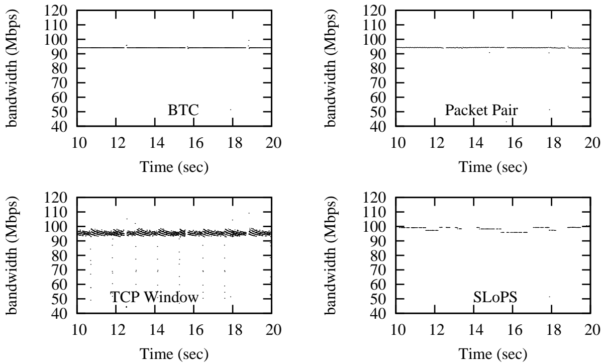
Figure 1. Techniques applied to iperf traffic monitored on uncongested 100 Mb LAN.
