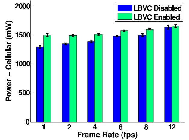
Fig. 4. Power Consumption vs. Frame Rate in a Cellular Network on Galaxy Nexus.
