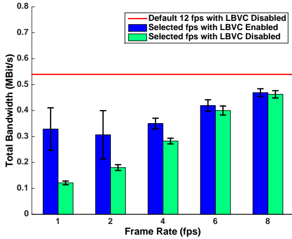
Fig. 3. Bandwidth Usage vs. Frame Rate on Galaxy Nexus.
