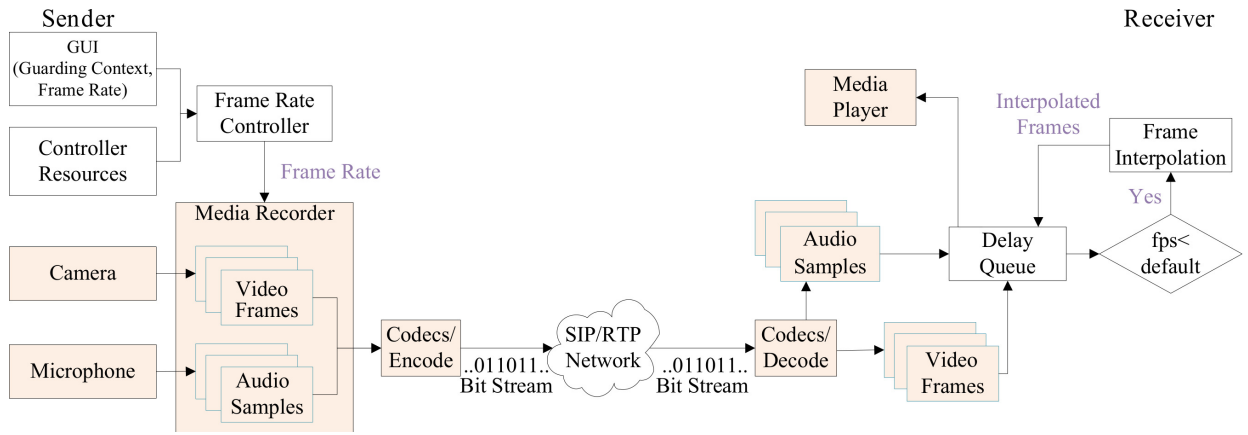
Fig. 1. LBVC Architecture.
