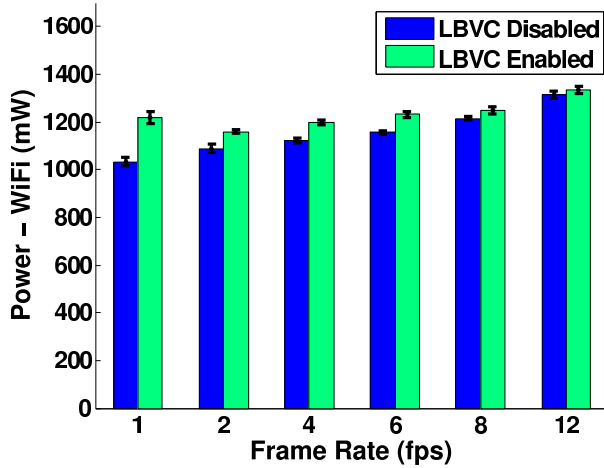
Fig. 5. Power Consumption vs. Frame Rate in a WiFi Network on Galaxy Nexus.
