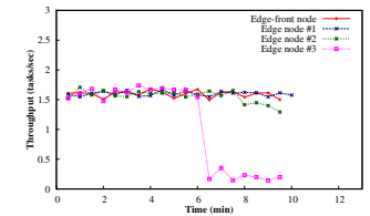
Fig. 5: Performance of SSLF.
