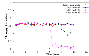
Fig. 4: Performance of SQLF.
