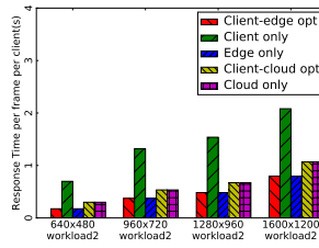
Fig. 2: The comparison of task selection impacts on edge offloading and cloud offloading for wired clients (RPi2).
