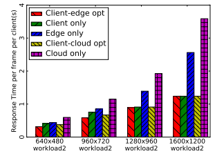
Fig. 3: The comparison of task selection impacts on edge offloading and cloud offloading for 2.4 Ghz wireless clients (RPi3).
