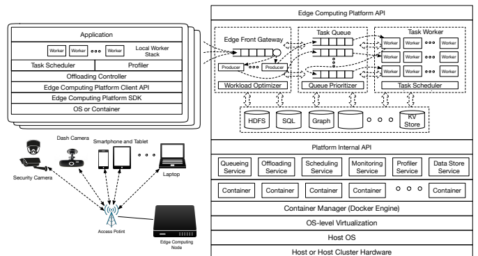
Fig. 1: The architecture of edge computing platform
