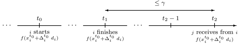
FIG. 3.2. Timeline for asynchronous pattern search message from process i to process j
