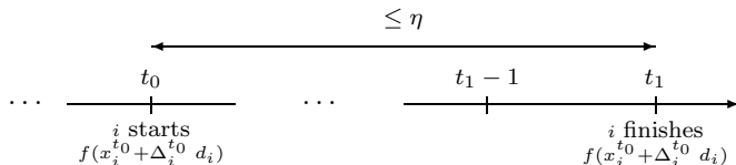
FIG. 3.1. Timeline for asynchronous pattern search on process i
