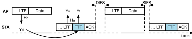
Fig. 7. MAC-layer operations of EliMO. The STA inserts Y_d in FTF and sends it to the AP along with LTF. Based on Y_u and Y_f , the AP estimates downlink CSI to calculate the beamforming matrix for the data packet.
