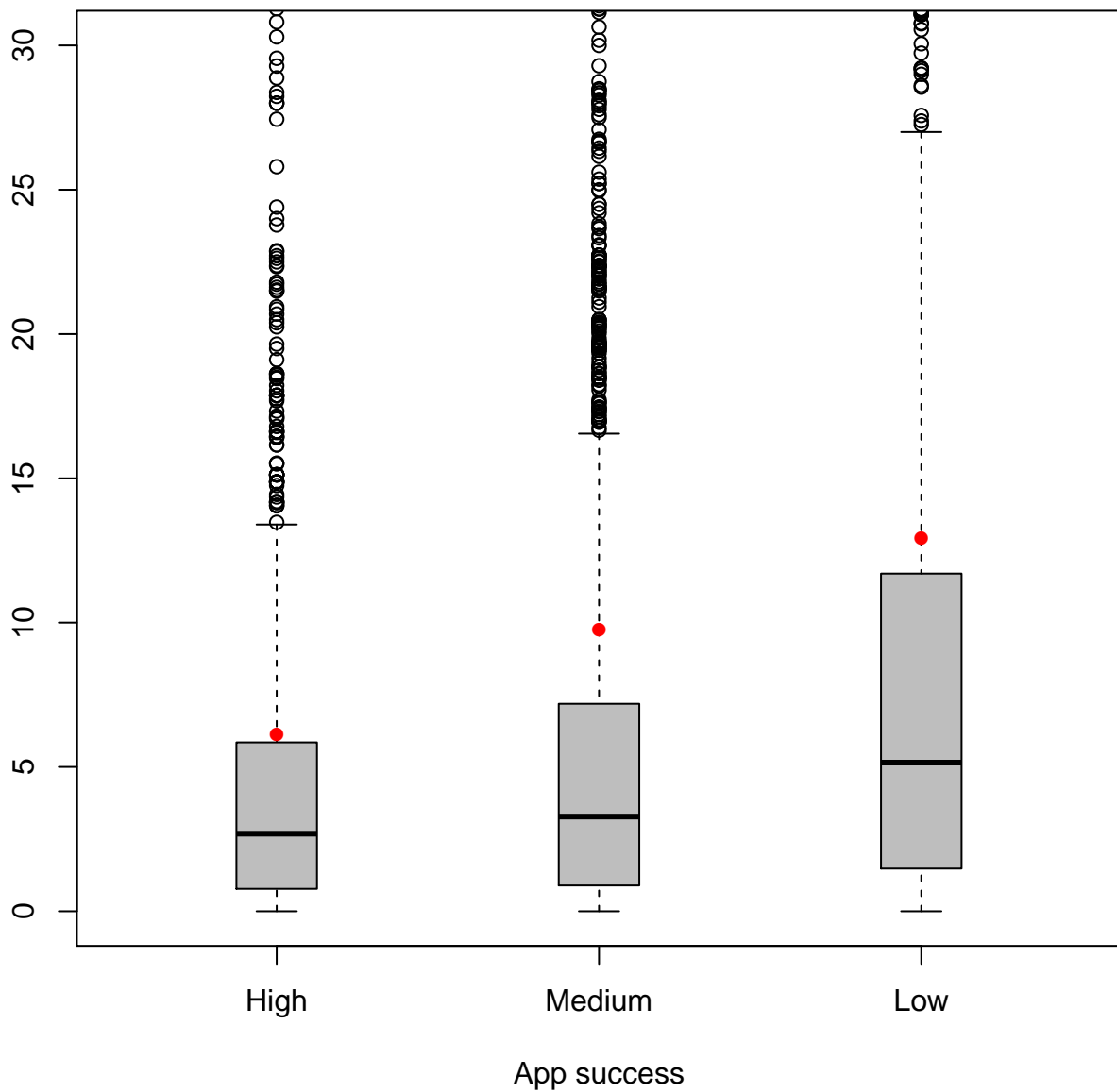
Average bug-fixes in used APIs
