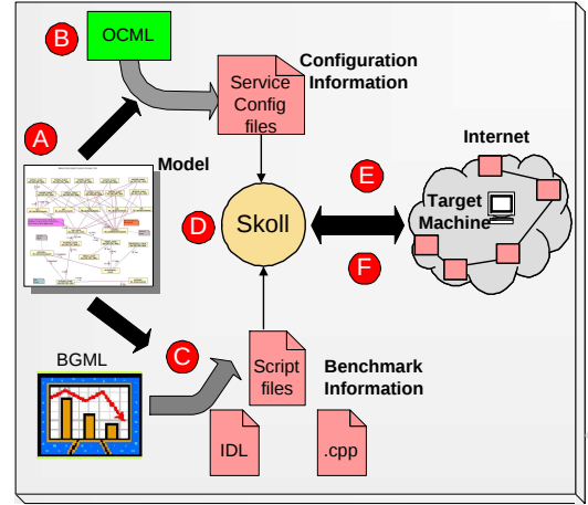
Figure 5: Alleviating C&C Patterns Validation Challenges via DCQA Processes
