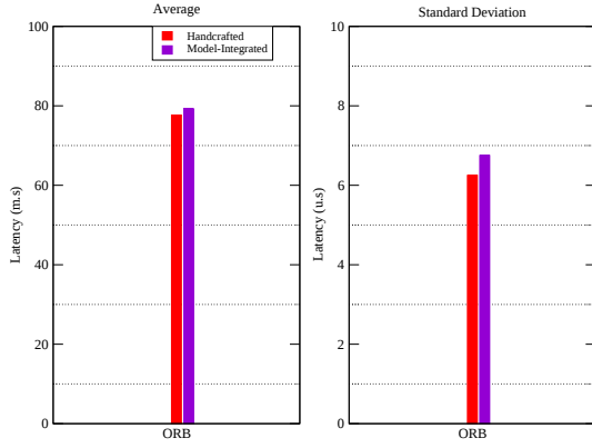
Figure 7: Execution Comparison
