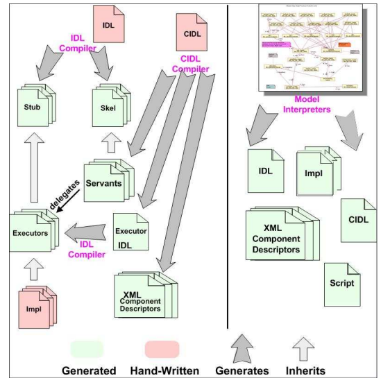
Figure 4: Code Generation Comparison in the Handcrafted vs. MDM Approaches
