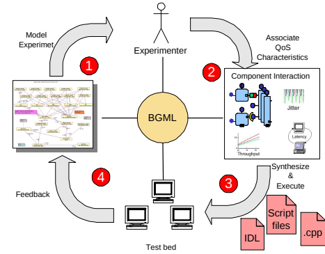
Figure 3: BGML Workflow
