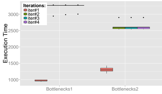
Fig. 5 Average execution times (in second) for different groups of injected bottlenecks (i.e.,bottlenecks#1 and bottlenecks#2), where n_p = 10 and n_u = 5 . Different colors represent different iterations. The central box represents the values from the lower to upper quartile (i.e., 25 to 75 percentile). The middle line represents the median.
