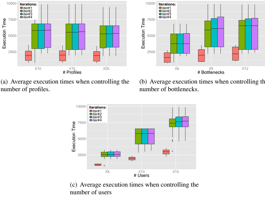
Fig. 6 Average execution times (in second) when controlling different independent variables. Different colors represent different iterations. The central box represents the values from the lower to upper quartile (i.e., 25 to 75 percentile). The middle line represents the median.
