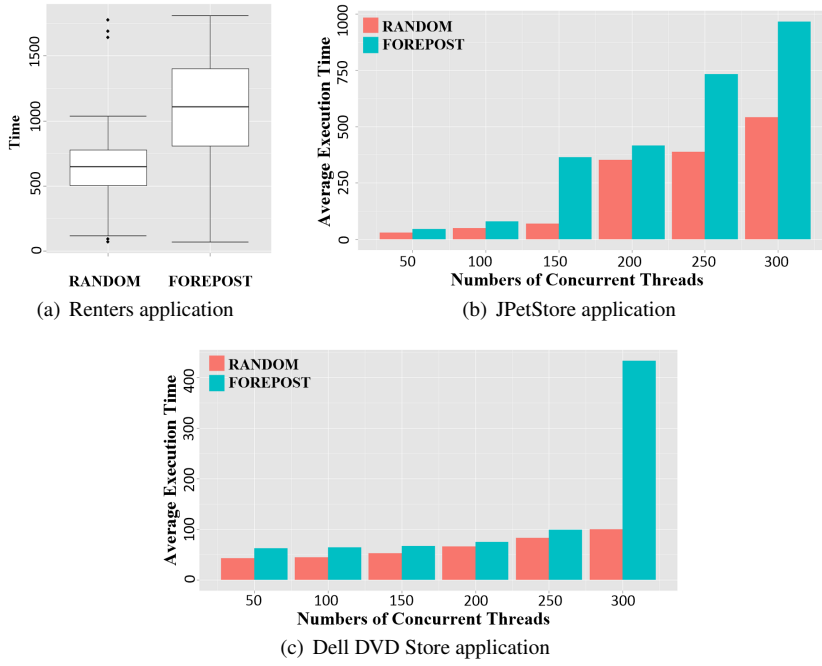
Fig. 4 The summary of the results for Empirical Study 1. The box-and-whisker plots for Renters are shown in Figure (a), where the time for end-to-end runs is measured in seconds. The central box represents the values from the lower to upper quartile (i.e., 25 to 75 percentile). The middle line represents the median. The thicker vertical line extends from the minimum to the maximum value. The bar graphs for JPetStore and Dell DVD Store are shown in Figure (b) and (c), where the bars represent average times per transaction in seconds for the Random and FOREPOST approaches for different numbers of concurrent transactions ranging from 50 to 300.
