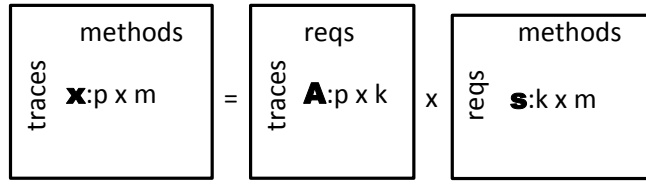
Fig. 2 Schematics of the ICA matrix decomposition.
