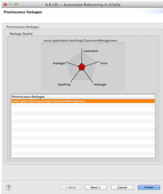
Fig. 1. Identification of Promiscuous Packages in ARIES
