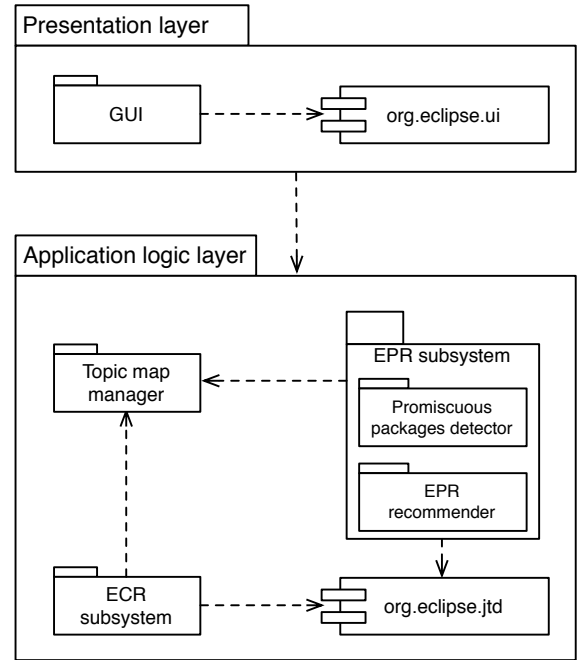
Fig. 4. ARIES Architecture
