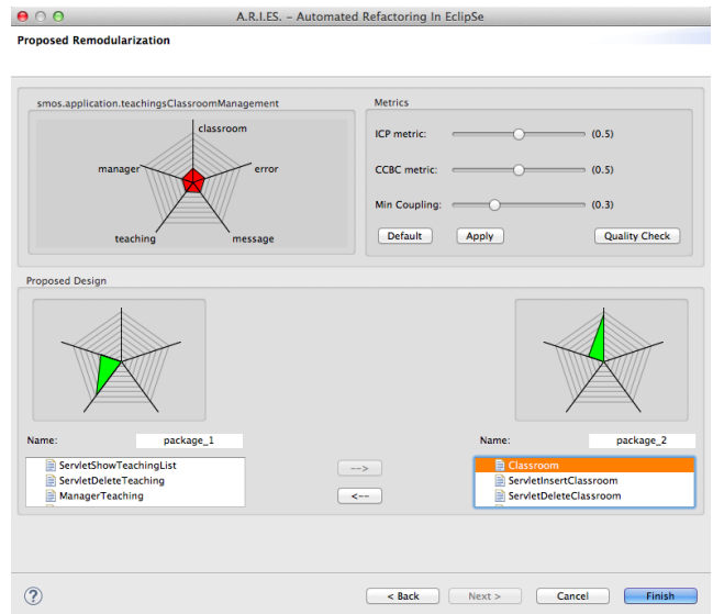
Fig. 2. Refactoring of a Promiscuous Package in ARIES
