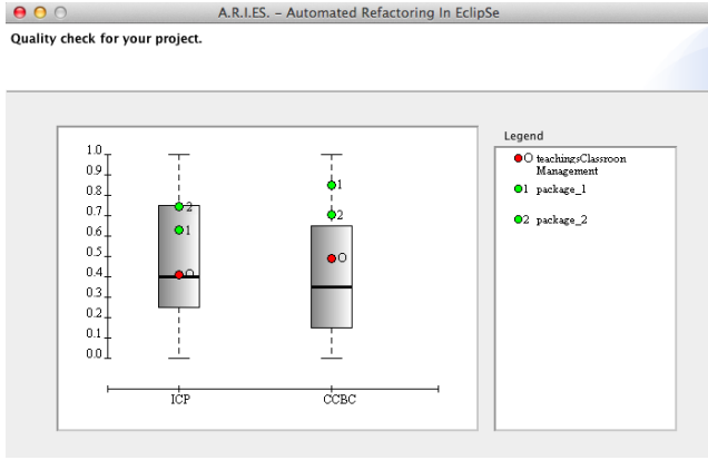
Fig. 3. Functionality Quality Check in ARIES
