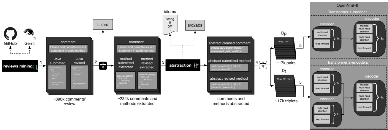
Fig. 1: Approach overview.
