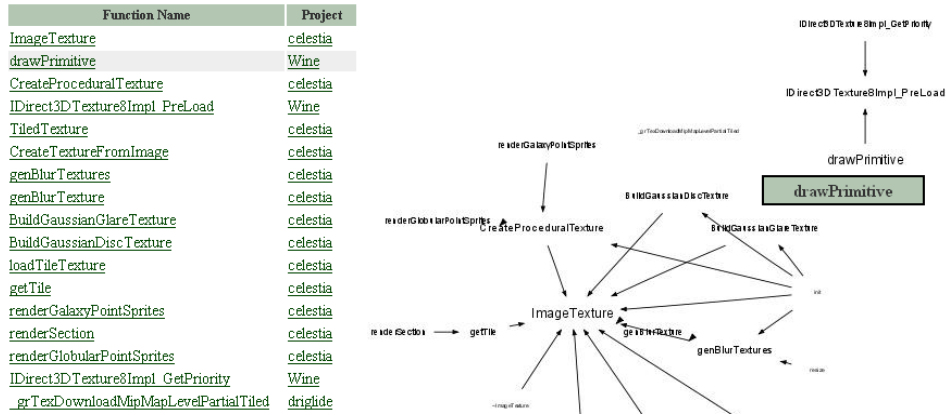
Figure 4: The visual interface of Portfolio. The left side contains a list of ranked retrieved functions for the motivating example query and the right side contains a call graph that contains these functions; edges of this graph indicate the directions of function invocations. Hovering a cursor over a function on the list shows a label over the corresponding function on the call graph. Font sizes reflect the score; the higher the score of the function, the bigger the font size used to show it on the graph. Clicking on the label of a function loads its source code in a separate browser window.
