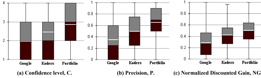
Figure 6: Statistical summary of the results of the first experiment for C, P, and NG. The central box extends from the lower to upper quartile. The thick white line is the mean. The thin black line is the median. The thin vertical line extends from the minimum to the maximum value.
