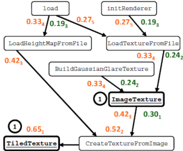
Figure 3: Example of SAN computation, w_{ij} = 0.8 . Weights that are computed starting with the function TiledTexture are shown in orange, and Weights that are computed starting with the function ImageTexture are shown in green.
