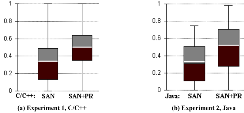
Figure 9: Normalized Discounted Cumulative Gain for Portfolio with PageRank enabled ( \text{Portfolio}_{\text{SAN+PR}} ) and disabled ( \text{Portfolio}_{\text{SAN}} ).
