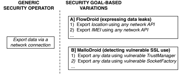
Figure 3: A generic “network export” security operator, and its more fine-grained instantiations in the context of FlowDroid [13] and MalloDroid [35].
