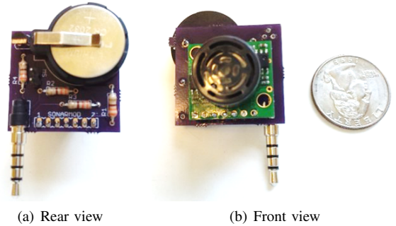
Fig. 1. Figure (a) is a picture of the 3.3V battery, the modulator circuit, and the male 3.5mm male headphone jack adapter. Figure (b) is a picture of the transducer module.
