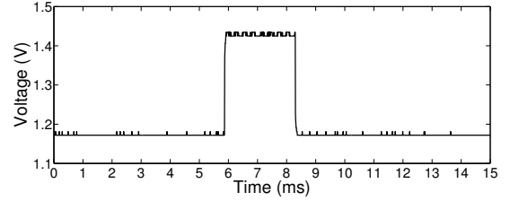
(b) Pulse-Width Modulated Signal
