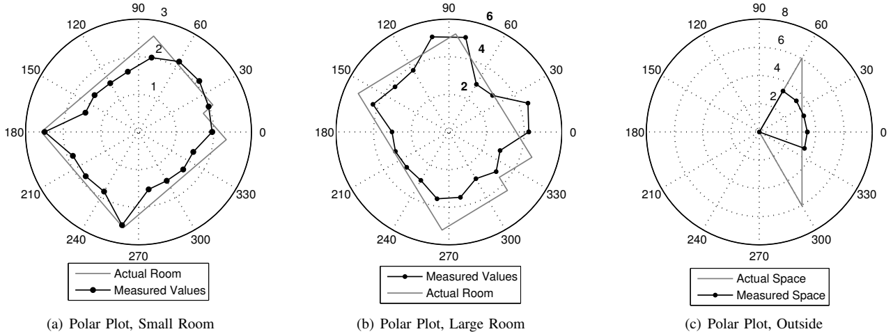
Fig. 10. Figures (a), (b) and (c) show the polar values obtained by the external SONAR module in a small room, a large room and outdoor environment, respectively. The application divides the compass into eighteen 20 degrees sections. A measurement taken in a given section will associate that value with the center of that section. All measurements shows are in meters and all angles are in degrees
