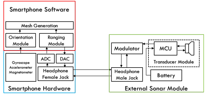
Fig. 2. Shows a system diagram of the proposed SONAR system, which is comprised of: 1) an external SONAR module; 2) a commodity smartphone; and 3) the software application running on the phone.
