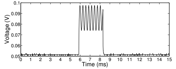
(c) Modulated Continuous Wave Signal
