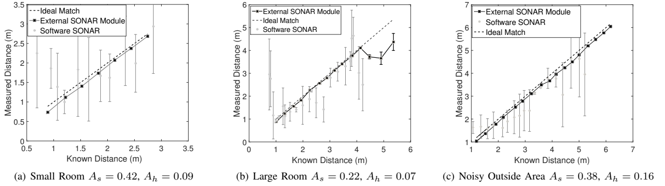
Fig. 9. Figures (a), (b), and (c) show the results for a small room, large room, and outside. Ten measurements were taken at each distance; the error bars represent the standard deviation of these measurements. A_s represents the average error for software SONAR module and A_h the average error for the software module.
