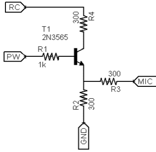
Fig. 4. Shows a circuit schematic of the modulation circuit. RC is the label for the received carrier. PW is the label for the pulse-width modulated signal. MIC is the label for the output of the modulator that is connected to the microphone input on the phone.
