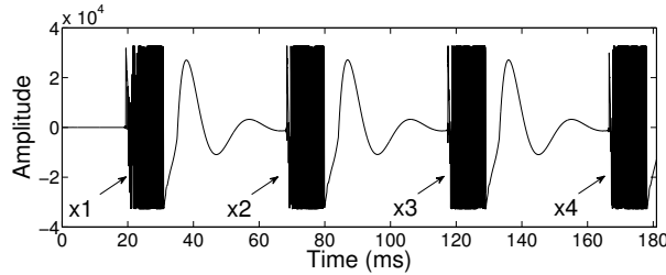
Fig. 6. Shows the 8000 samples obtained from a single reading of the buffer.
