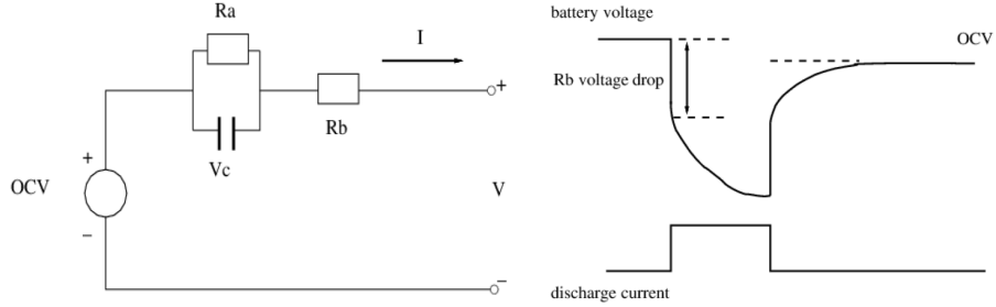
Figure 1: Battery voltage dynamics. Left: Equivalent electrical circuit model for batteries. Right: Battery voltage curve when discharge current is changed. The deep drop of voltage is caused by current increasing on resistor R_b .
