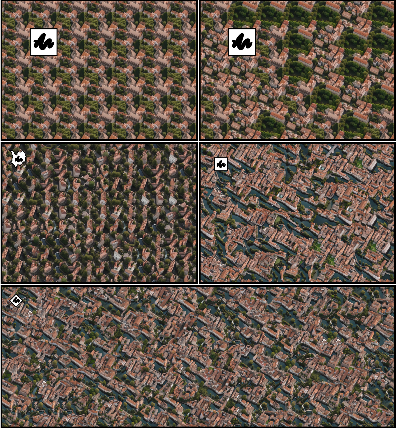
Fig. 8. Comparison of Tiling Schemes: A comparison of the different tiling schemes (first row: self-tiling and stochastic self-tiling (with 4 tiles); second row: stochastic Escher self-tiling (with 4 tiles) and regular 3-color Wang tiling (81 tiles); last row: 3-color Dual Wang tiling) demonstrated on texture tiles generated with the prompt “ European city blocks, tile roofs, streams, drone footage ”. For each example we also show the tile shape and size with the scribbled overlay.
