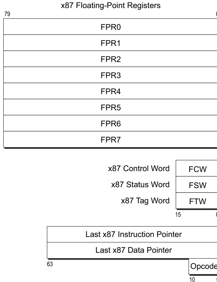
Figure 11-3. x87 Execution Unit State
