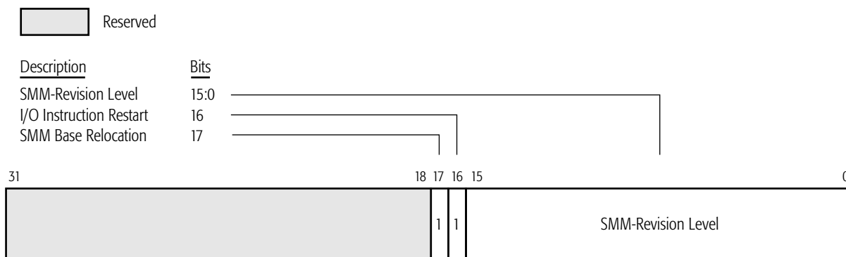
Figure 10-3. SMM-Revision Identifier
