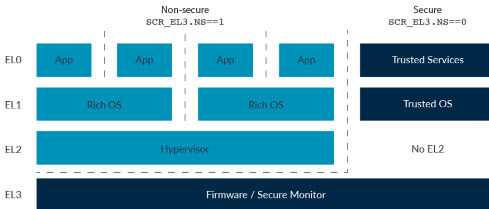
Figure 3-11: Secure virtualization
