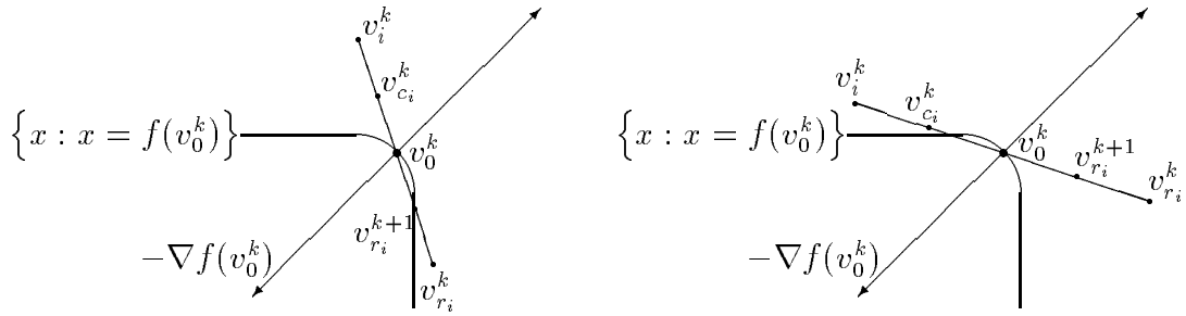
Figure 3.1 The two cases which guarantee a direction of descent
