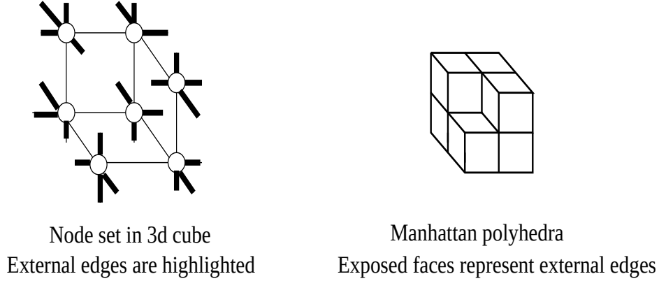
Figure 3: Geometric interpretation of a connected node set
